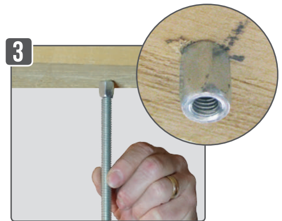
Install the M10 threaded rod
