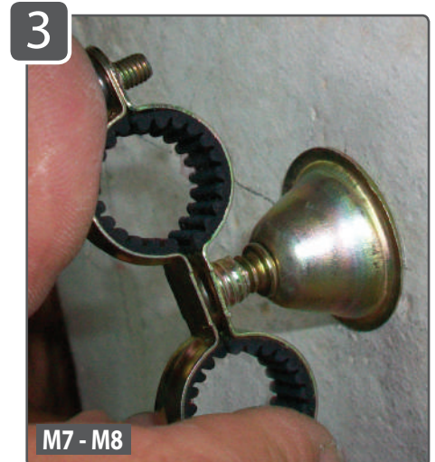
UNSCREWING POSSIBLE
