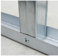
Vis ossature plaque de plâtre - montant + rail
